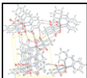
Fig. 2. The crystal packing of the title compound in the unit cell. The hydrogen bonds were shown dashed lines.
